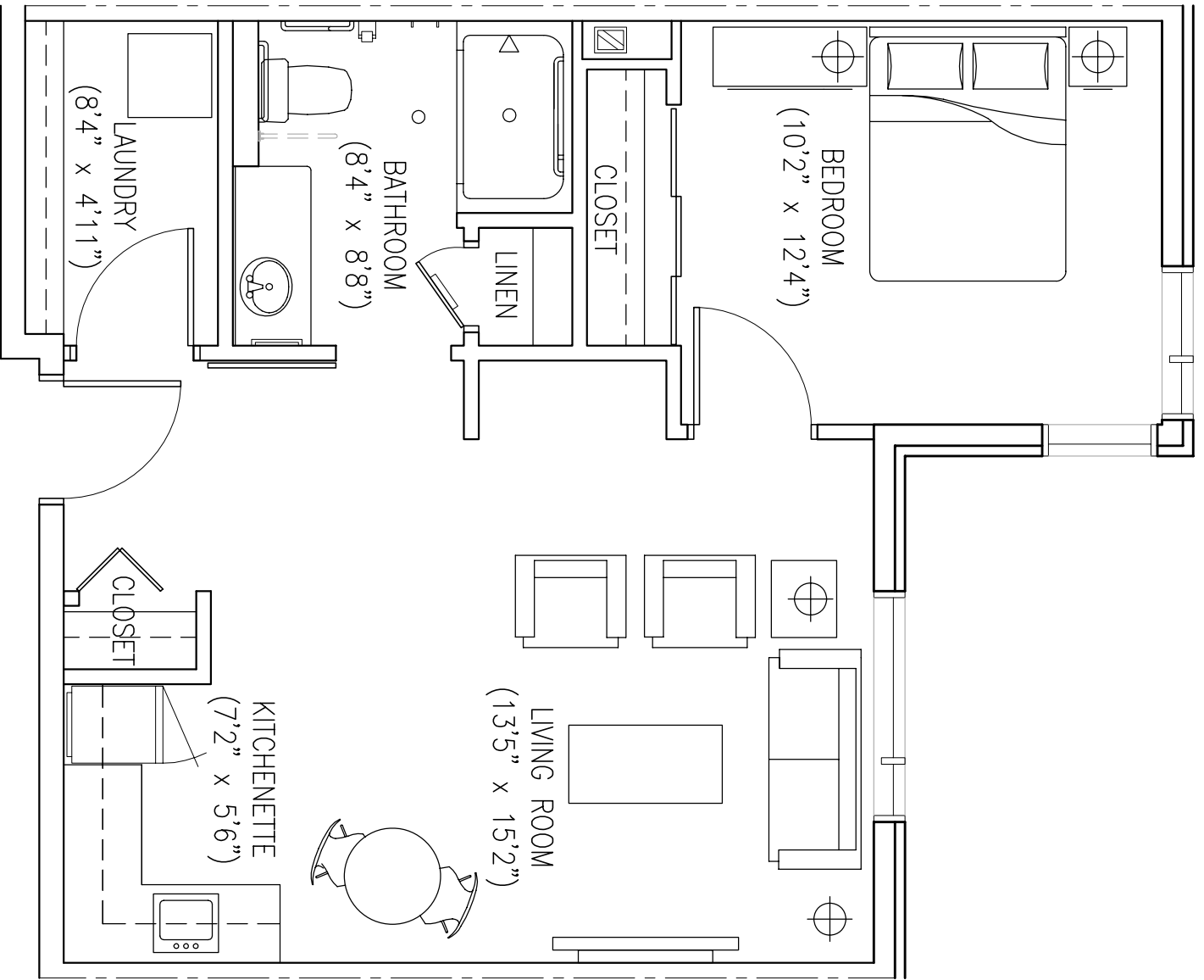
UNIT - TYPE B 1:50
